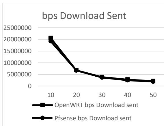
Gambar 3. Grafik Throughput Unduh
