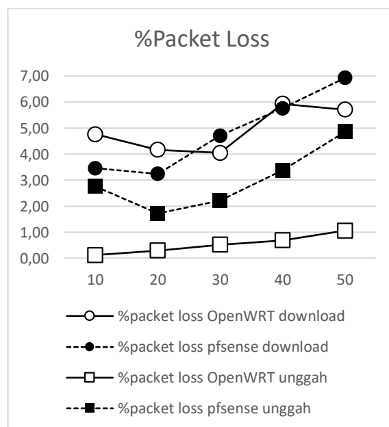
Gambar 9. Persentase Packet Loss
