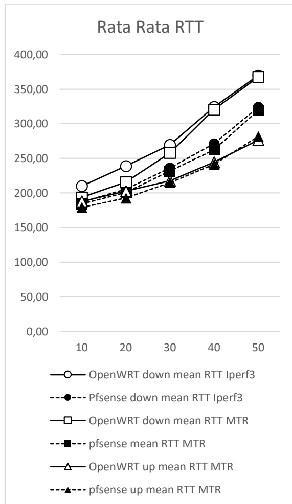
Gambar 5. RTT Rata Rata OpenWRT dan PfSense
