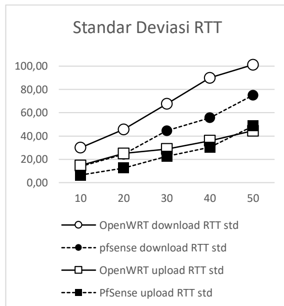
Gambar 8. Standar Deviasi RTT
